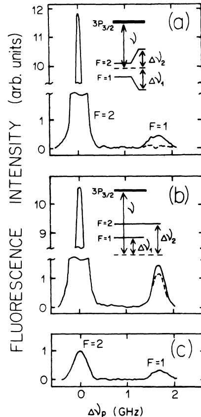
FIG. 2. Quantum-state-selective reflection of atomic sodium beam at atomic mirror. (a) Absorption spectrum of reflected atomic beam at detunings of intense laser field forming atomic mirror [\omega_1 - (\omega_{10} + k_1 v_p)]/2\pi = -1.2 GHz, [\omega_2 - (\omega_{20} + k_1 v_p)]/2\pi = +0.5 GHz ( v_p = 8.2 \times 10^4 cm/s). (b) Same for the case \Delta\omega_1/2\pi = +2.9 GHz, \Delta\omega_2/2\pi = +4.6 GHz. (c) Same at P_L=0 (scattered atoms). Dashed line, result of subtraction of background signal due to scattered atoms.
