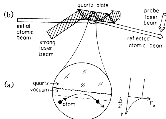
FIG. 1. (a) Principle of mirror reflection of atoms by nonuniform laser field of surface wave. (b) Schematic diagram of experimental setup.
