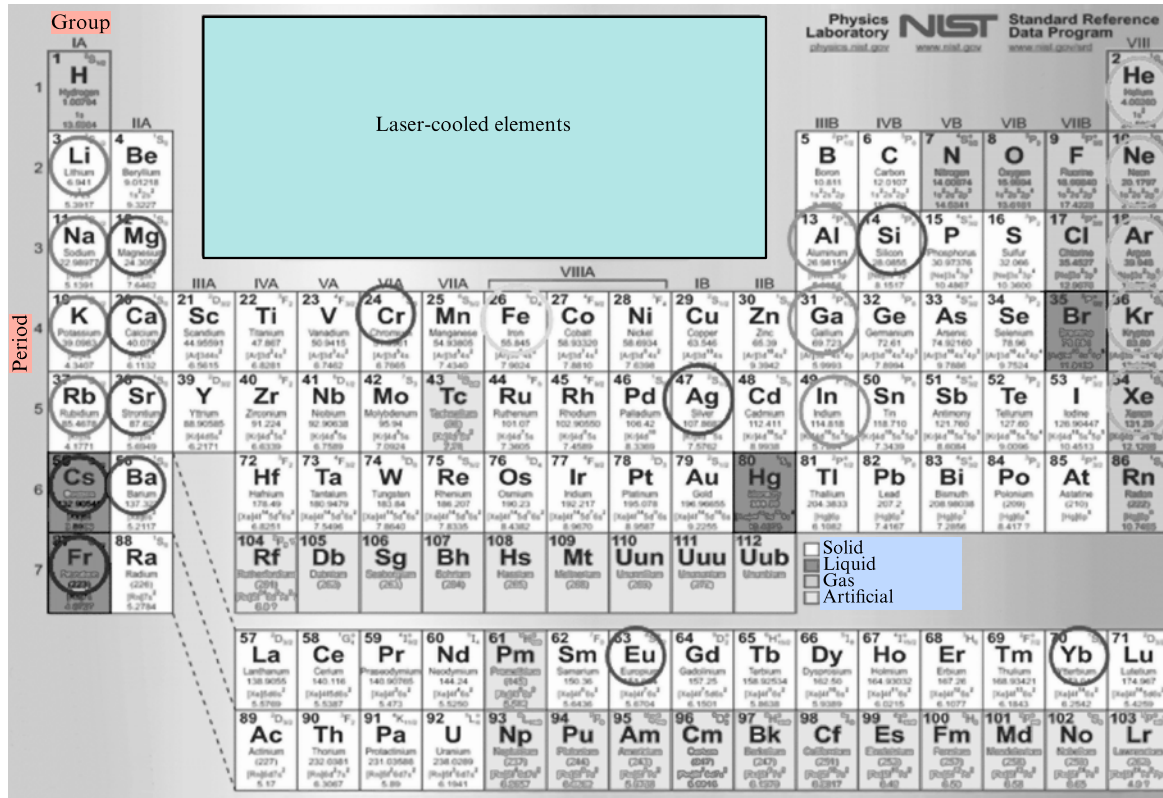
Figure 2. Elements (marked by circles) of the periodic table for which laser cooling of atomic beams has been carried out.
