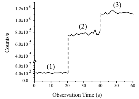
FIG. 2: Photon count through the optical fiber under three conditions; (1) both MOT laser beams and B-fields are switched off, (2) MOT laser beams are switched on, and (3) both MOT laser beams and B-fields are switched on.
