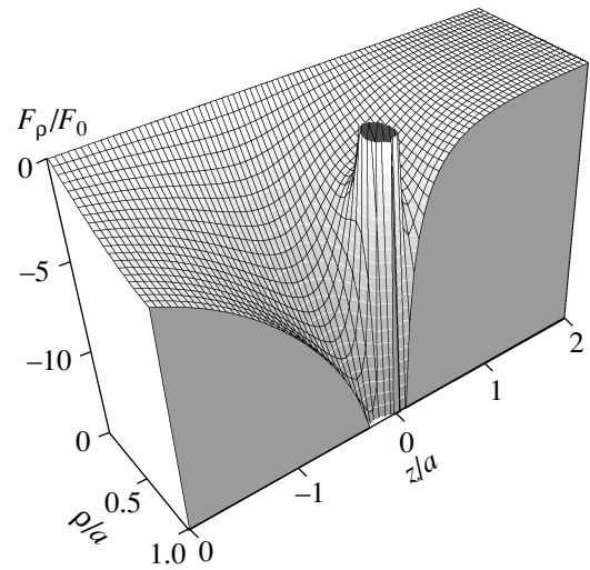
Fig. 5. Radial force as a function of atomic coordinates in the case of incidence of circularly polarized radiation on a screen with an aperture for detuning \delta = -10\gamma and for relative aperture ka = 0.25 .
