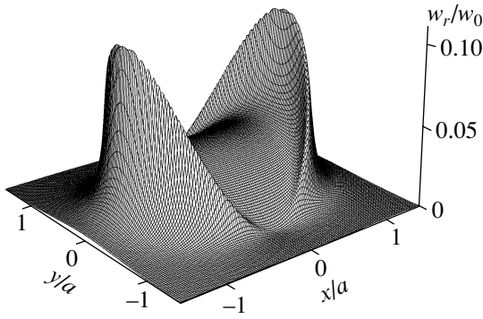
Fig. 2. Electric energy density as a function of transverse coordinates in the case of incidence of linearly polarized radiation on a screen with a circular aperture for ka = 0.25 and at a distance z = 0.05a from the aperture.
