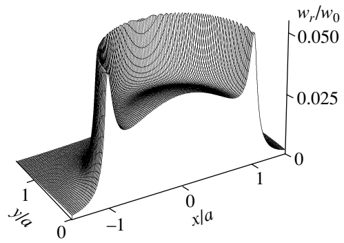
Fig. 3. Electric energy density as a function of transverse coordinates in the case of incidence of circularly polarized radiation on a screen with a circular aperture for ka = 0.25 and at a distance z = 0.05a from the aperture.
