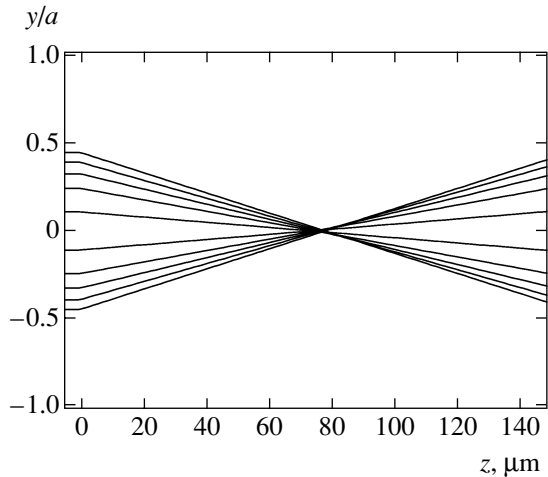
Fig. 7. Trajectory of atoms in the longitudinal cross section of an atomic beam before and after its passage through an atomic microlens in the case of blocking of atoms propagating in the region 0.5a < r < a by a circular screen for the same values of parameters as in Fig. 6.
