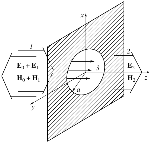
Fig. 1. Atomic optical near-field microlens: the field to the left of the screen, produced by incident radiation and radiation reflected from the aperture (1); the field to the right of the screen, formed by radiation transmitted through the aperture (2); atomic beam being focused (3).
