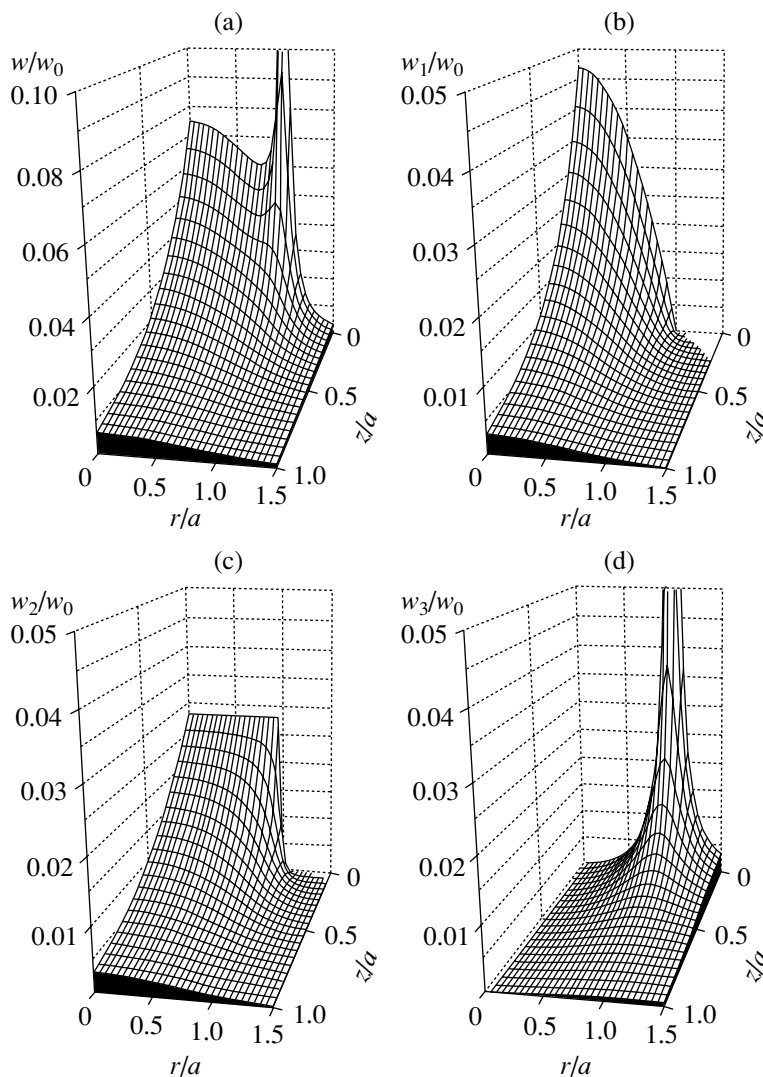
Fig. 4. (a) Electric energy density as a function of coordinates in the case of incidence of circularly polarized radiation on a screen with a circular aperture for ka = 0.25 . The contributions from the first (b), second (c), and third (d) terms of relation (32) to the total energy density.
