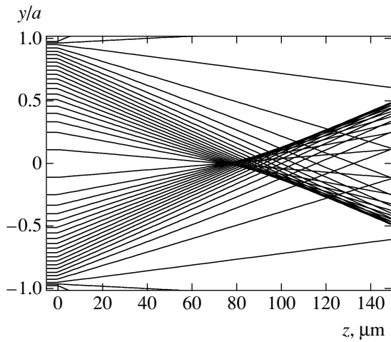
Fig. 6. Trajectory of atoms in the longitudinal cross section of a monochromatic atomic beam before and after its passage through an atomic microlens. The screen with an aperture is illuminated by circularly polarized radiation with detuning \delta = -300\gamma and intensity I = 16 \text{ W/cm}^2 . The relative aperture is ka = 0.5 . The longitudinal velocity of atoms is v_z = 1200 \text{ cm/s} .
