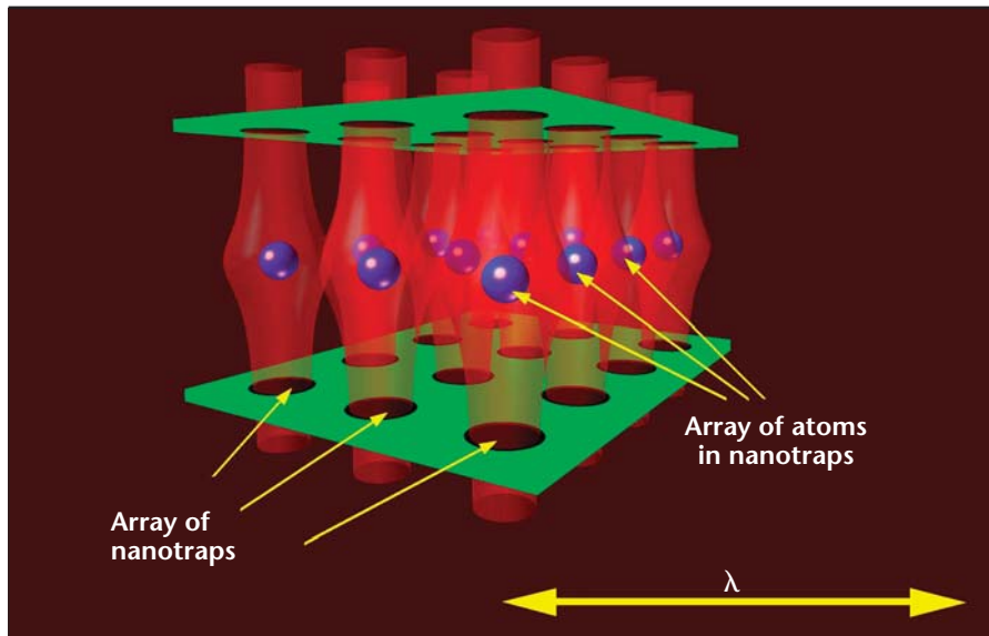
Figure 5. Array of atomic traps. Trapping of atoms in nanometer-sized regions spaced at distances much smaller than the wavelength of light.
