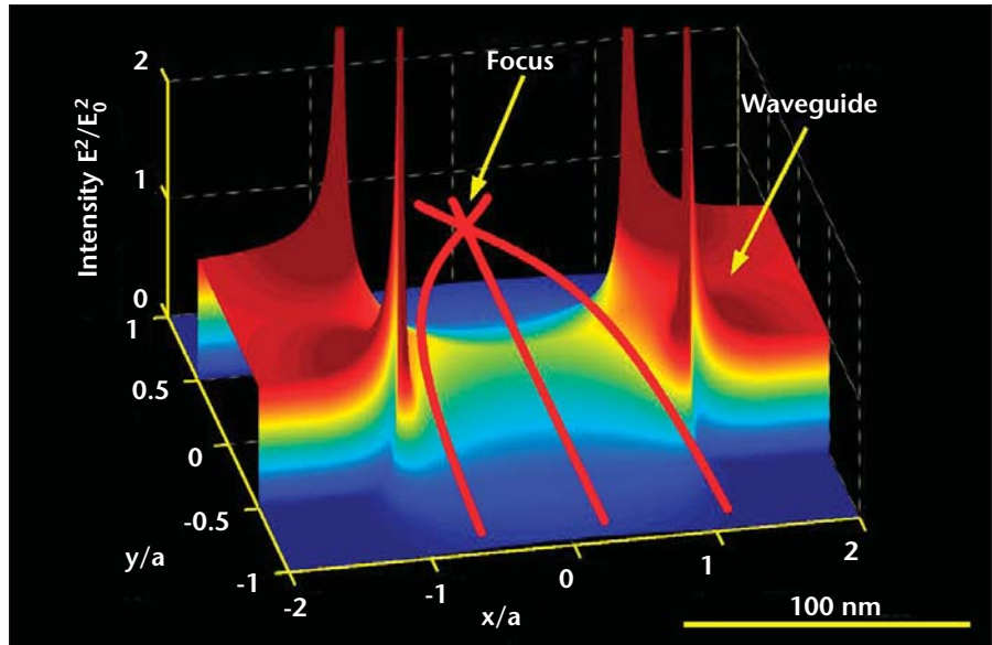
Figure 2. Focusing of atom waves. Light field intensity distribution near the apertures inside and outside the subwavelength-thickness waveguide and trajectories of slow atoms. The thickness of the waveguide is equal to the radius of the apertures.
