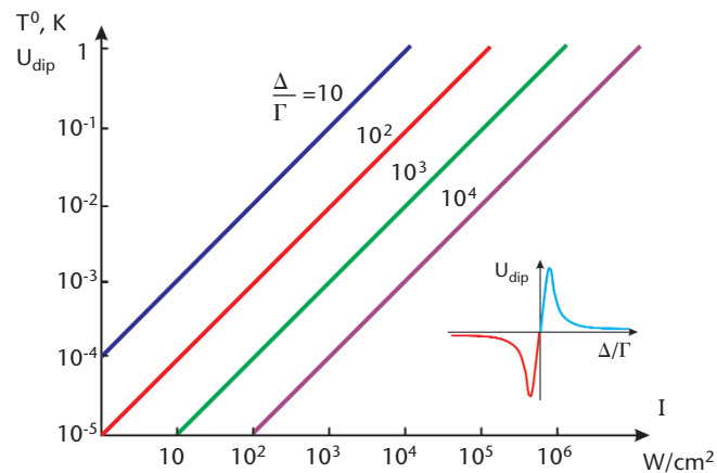
Figure 3. Dependence of potential energy U_{\text{dip}} of the dipole on radiation intensity I=\frac{c}{8\pi}E^2 and detuning \Delta/\Gamma of field frequency \omega relative to resonance frequency \omega_0 .
