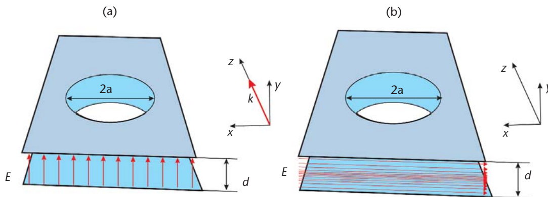
Figure 1. Plane waveguide and light field E orientation for (a) photon dots and (b) photon holes.
