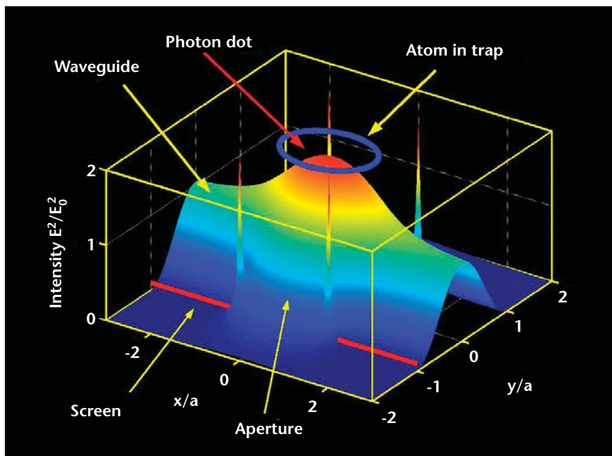
Figure 4. Light field intensity distribution near the apertures inside and outside the waveguide when the electrical strength vector is parallel to the waveguide-photon dot. The thickness of the waveguide is equal to the radius of the apertures. The photon dot forms a trap for an orbiting atom.
